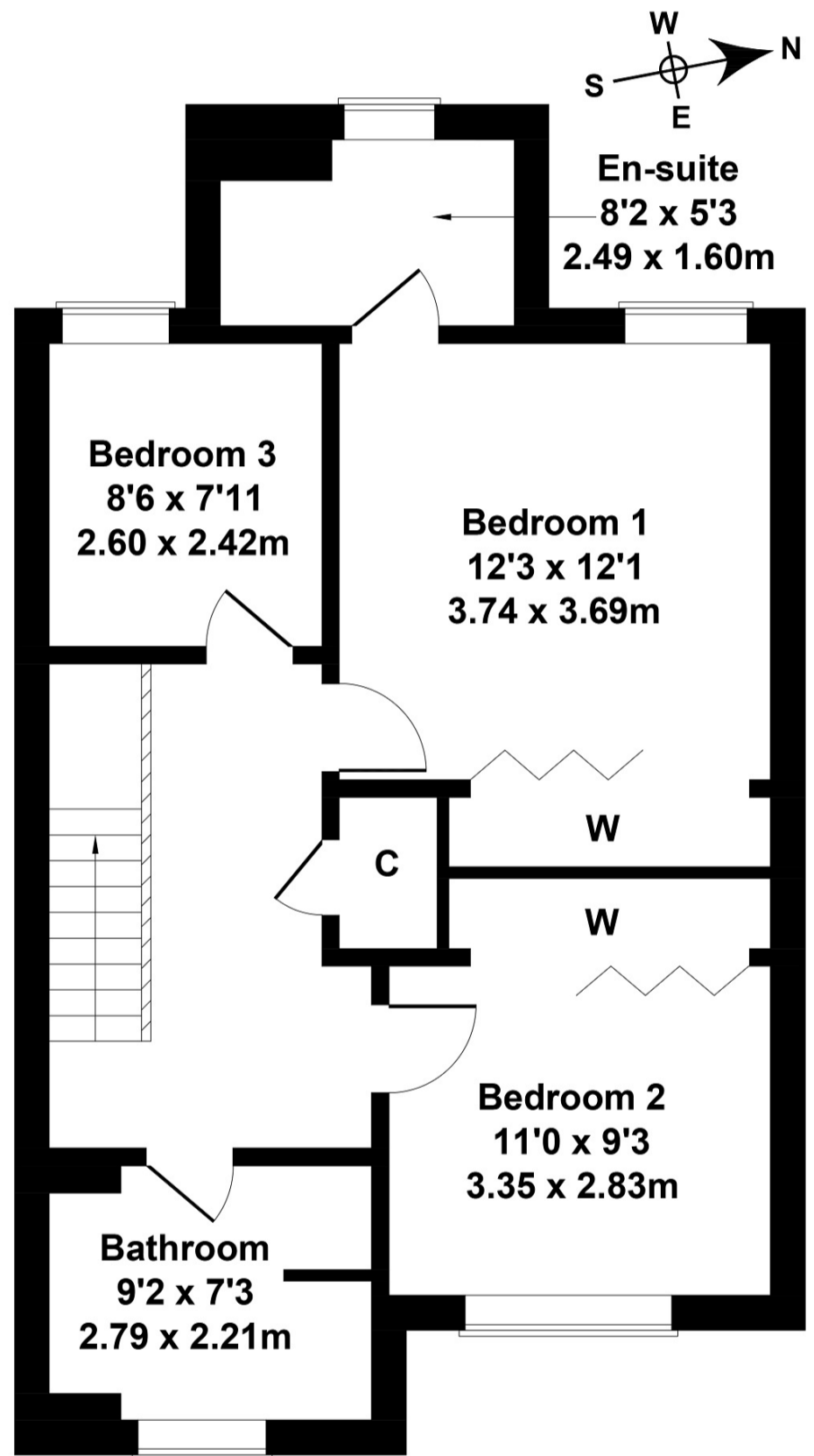
First Floor
